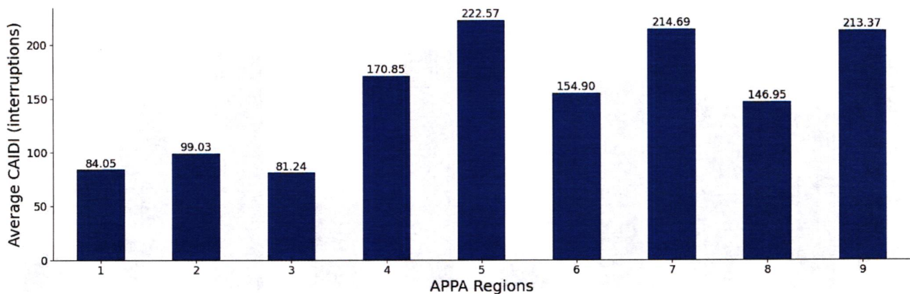
Figure 5. Average CAIDI for all utilities that use the eReliability Tracker by region
